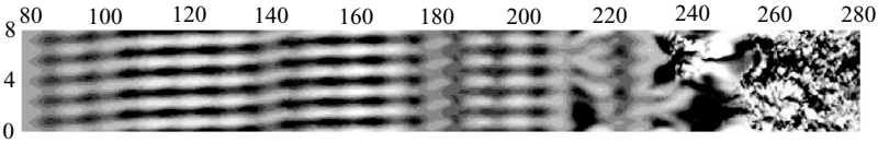
FIGURE 22. The contour of the streamwise fluctuation of the mode 5 case; t = 5\tau ; y = 0.5\delta_{99} . The spanwise coordinate is enlarged by a factor of 3. Contours are plotted in -0.2 < u < 0.2 .
