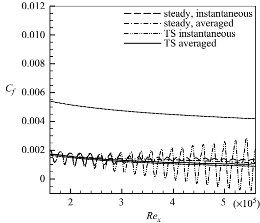
FIGURE 39. The skin friction curves for cases with steady and unsteady streaks, mode 5, A_{TS}^0 = 1.0\% , A_{con}^0 = 2.1\% .
