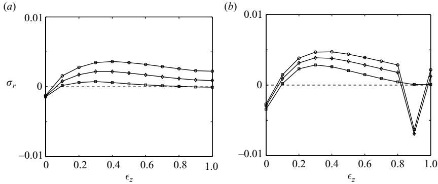
FIGURE 35. Effect of the spanwise detuning factor \epsilon_z on the growth rate of the (a) fundamental and (b) the subharmonic (in x ) instability of mode 5. The streak amplitude, B = 10\% . Three T-S wave amplitudes are shown: \square , A = 1.5\% ; \diamond , A = 2.0\% ; \circ , A = 2.5\% .
