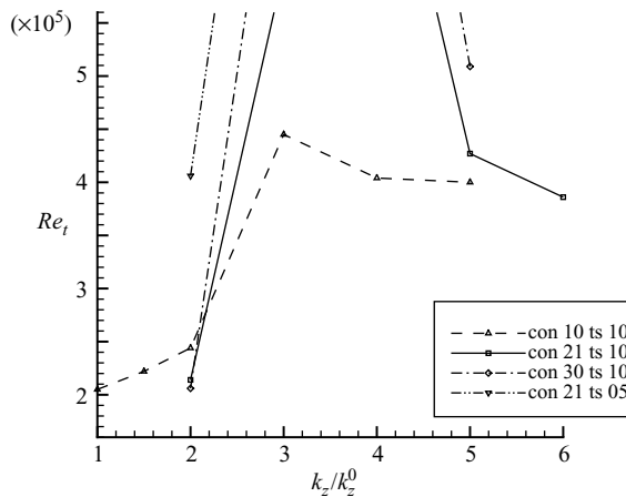
FIGURE 37. A graphical illustration of table 5. Decaying cases are treated by setting a large value to Re_t .
