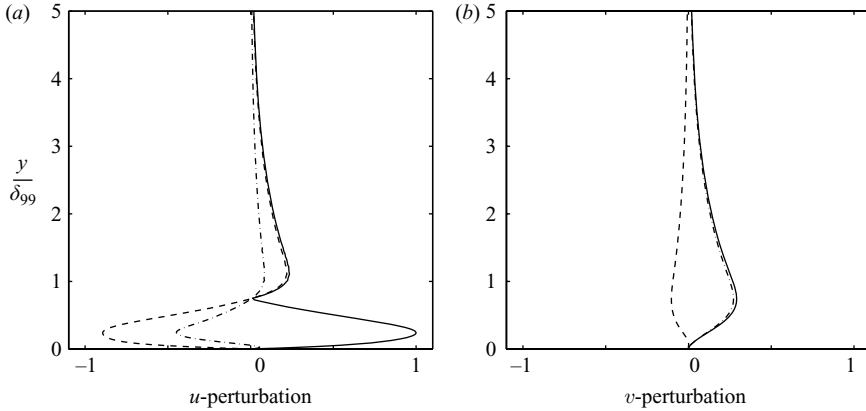
FIGURE 2. Profile of the T-S mode. The (a) u -component, and (b) the v -component. —, mode amplitude; - - -, real part; —·—, imaginary part.
