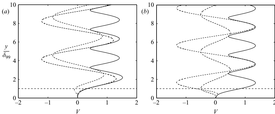
FIGURE 5. Profiles of (a) v and (b) \eta for mode 2. —·—, real; - - -, imaginary; —·—, ABS.
