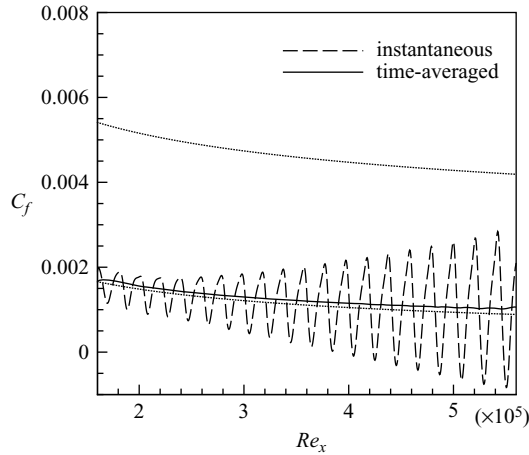
FIGURE 4. The skin friction coefficient vs. the Re_x ; t = 3\tau . - - -, instantaneous; —, time averaged (Blasius is shown by dotted line); ..., turbulent.
