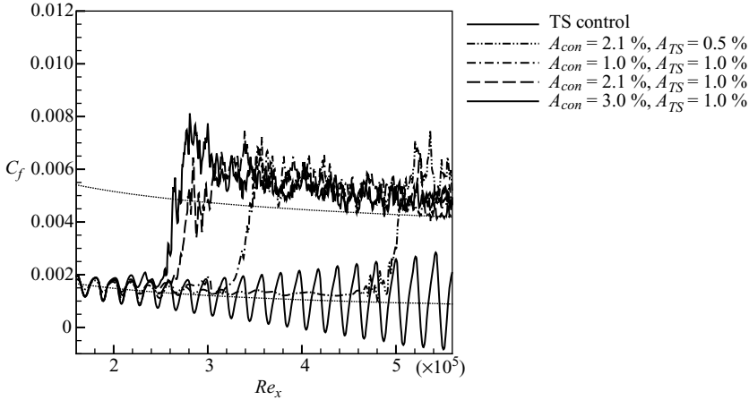
FIGURE 18. The skin friction of mode 2; effects of disturbance energy.
