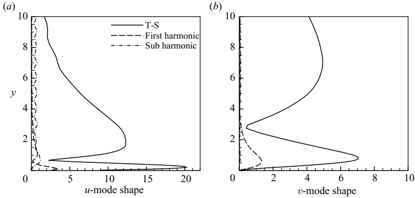
FIGURE 33. Profiles of (a) the streamwise and (b) wall-normal spectra.
