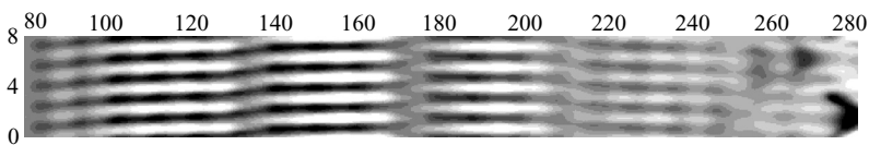
FIGURE 31. The contour of the streamwise fluctuation of the mode 5 case; A_{TS}^0 = 1.0\% , A_{con}^0 = 3.0\% ; t = 3\tau ; y = 0.5\delta_{99} .
