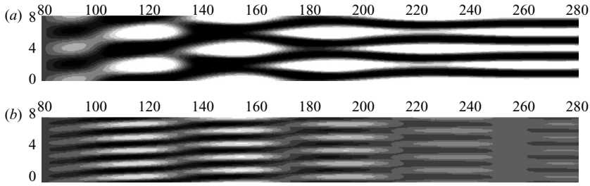
FIGURE 6. Contours of the streamwise velocity perturbation inside the boundary layer owing to inflow perturbation by (a) mode 2 and (b) mode 5; t = 3\tau ; y = 0.5\delta_{99} . The spanwise coordinate is enlarged by a factor of 3. Contours are plotted in -0.2 < u < 0.2 .
