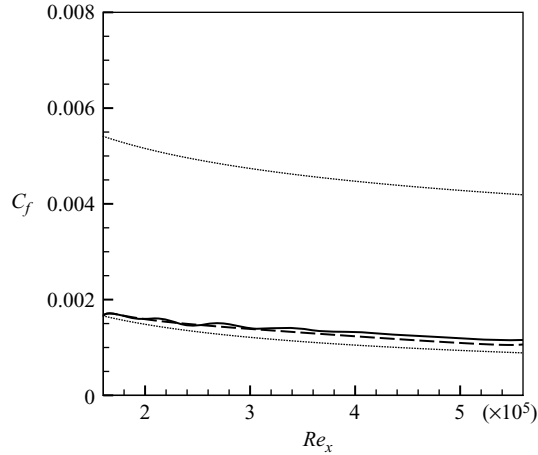
FIGURE 8. The skin friction coefficient vs. the Re_x ; t = 3\tau . —, instantaneous; - - -, time averaged; . . . , turbulent.
