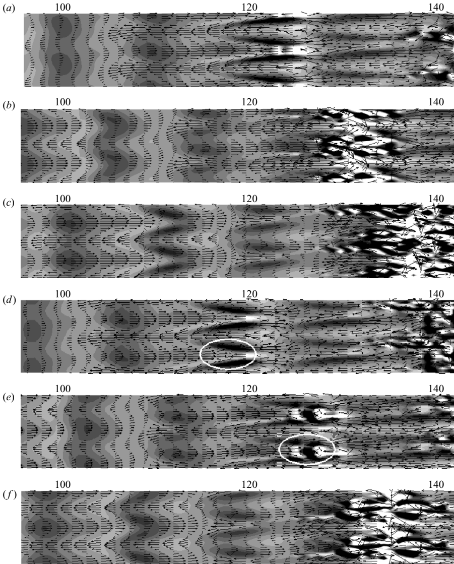
FIGURE 14. The instantaneous contour of the normal fluctuation and the vector plot of inplane components of the mode 2 case in the (x, y) -plane; y = 0.5\delta_{99} . Contours are plotted in -0.02 < v < 0.02 . Each frame is separated by \Delta t \sim 0.075\tau , where \tau is the flow-through time. The spanwise coordinate is not enlarged.
