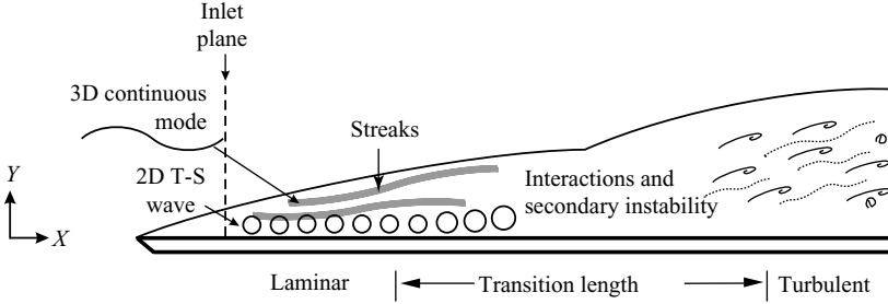
FIGURE 1. Schematic of the discrete-continuous mode interaction. The dashed line marks the boundaries of the computational domain.
