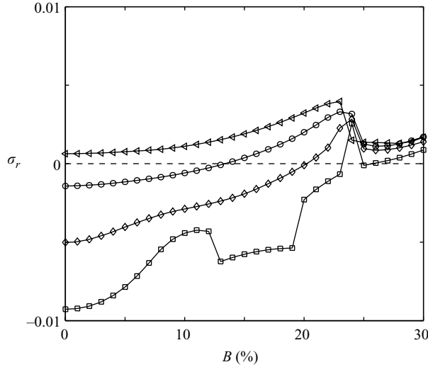
FIGURE 34. Effect of the streak strength B of mode 2 on the growth rate \sigma_r . The subharmonic instability in x ( NA=1 ) and fundamental in z ( NB=2 ) is considered at different amplitudes of the T-S waves: \square , A=0.2\% ; \diamond , A=0.5\% ; \circ , A=1.0\% ; \triangleleft , A=1.5\% .
