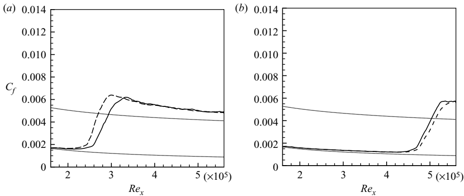
FIGURE 10. Skin friction coefficient for the spanwise domain size test of (a) mode 2 and (b) mode 5. Parameters are summarized in §§ 3 and 4. —, L_z = 8 ; ---, L_z = 12 .
