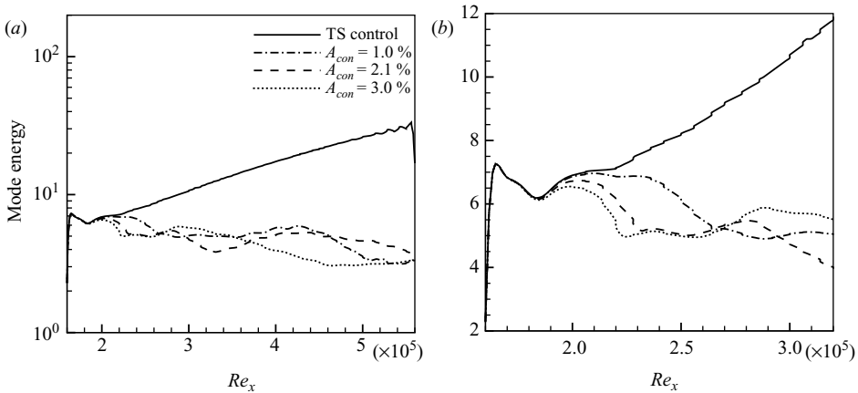
FIGURE 19. The amplitude of the fundamental T-S mode frequency for mode 2. A close up is shown in (b).
