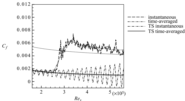
FIGURE 12. The skin friction coefficient vs. the Re_x of the mode 2 case. The lower curves show the T-S only case for reference; t = 3\tau .
