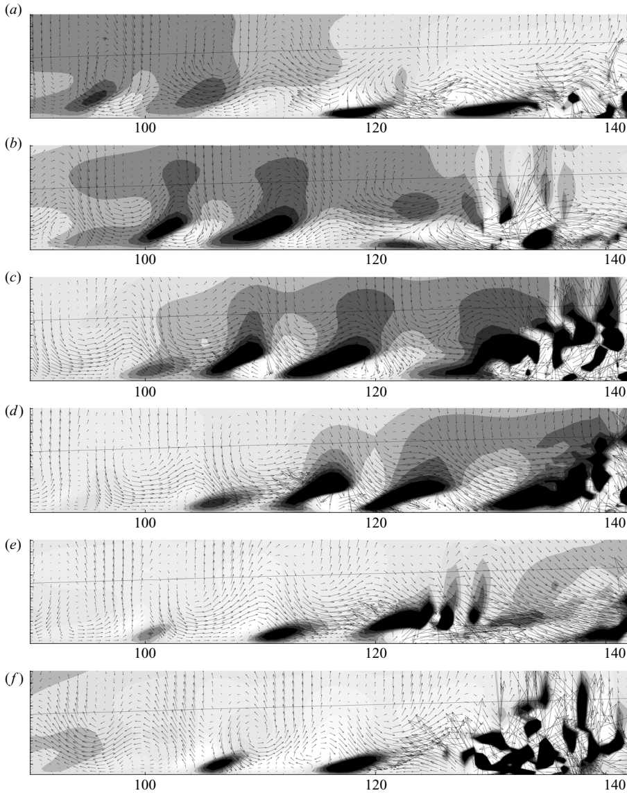
FIGURE 15. The instantaneous contour of the spanwise fluctuation and the vector plot of inplane components of the mode 2 case in the (x, y) -plane; the slice cuts through the centre of \Lambda -structures. Snapshots are taken corresponding to figures 13 and 14.
