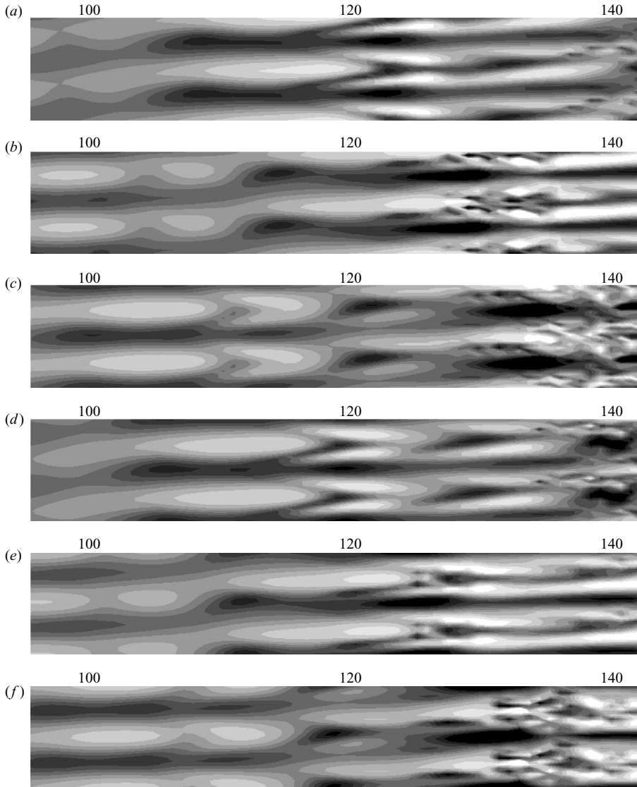
FIGURE 13. The instantaneous contour of the streamwise fluctuation of the mode 2 case in the (x, y) -plane; y = 0.5\delta_{99} . Contours are plotted in -0.2 < u < 0.2 . Each frame is separated by \Delta t \sim 0.075\tau , where \tau is the flow-through time. The spanwise coordinate is not enlarged.
