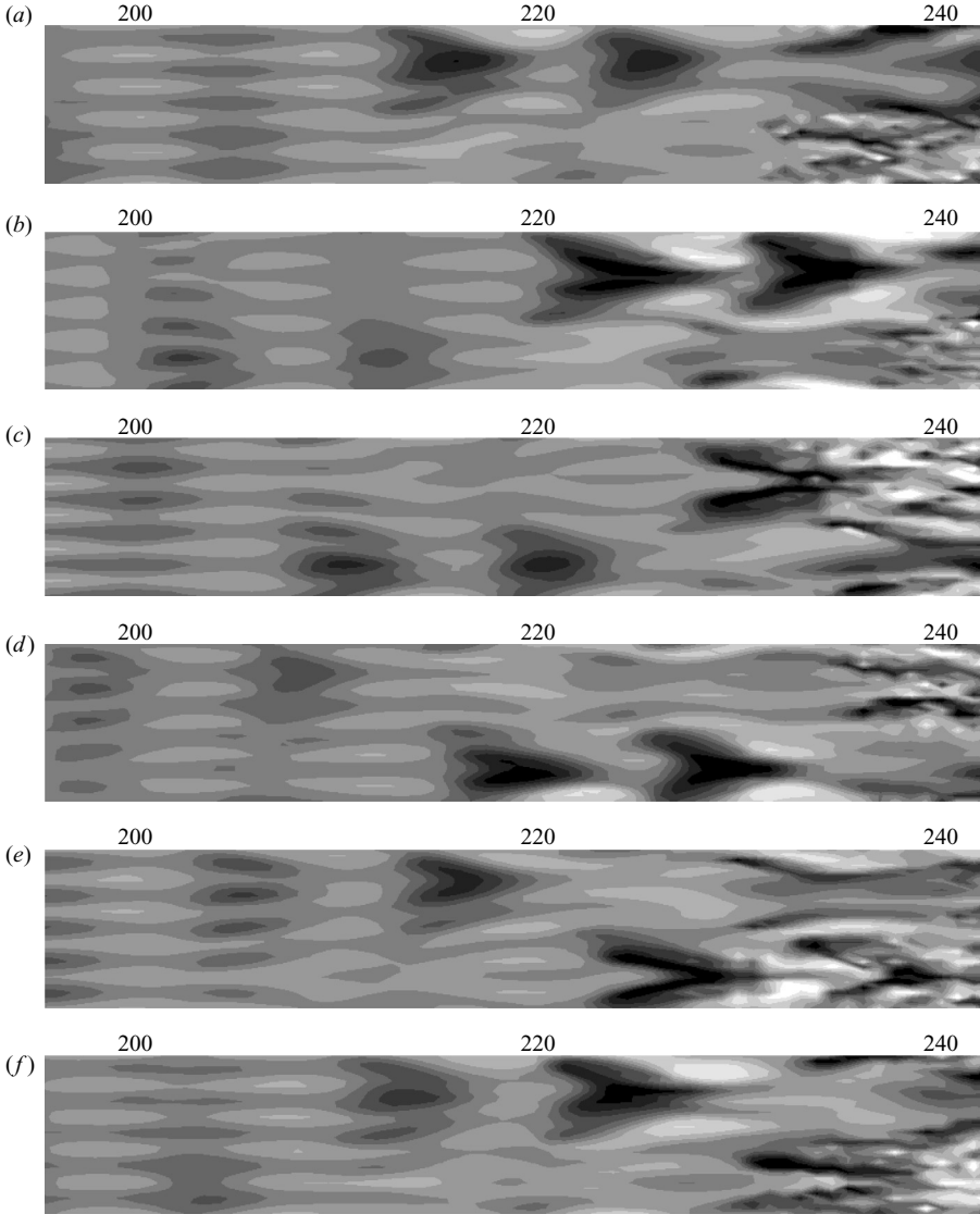
FIGURE 24. The instantaneous contour of the streamwise fluctuation of the mode 5 case in the (x, y) -plane; y = 0.5\delta_{99} . Contours are plotted in -0.2 < u < 0.2 . Each frame is separated by \Delta t \sim 0.1\tau , where \tau is the flow-through time. The spanwise coordinate is not enlarged.
