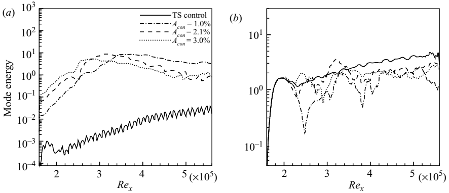
FIGURE 21. The amplitude of (a) the subharmonic and (b) first harmonic modes of the T-S perturbation.
