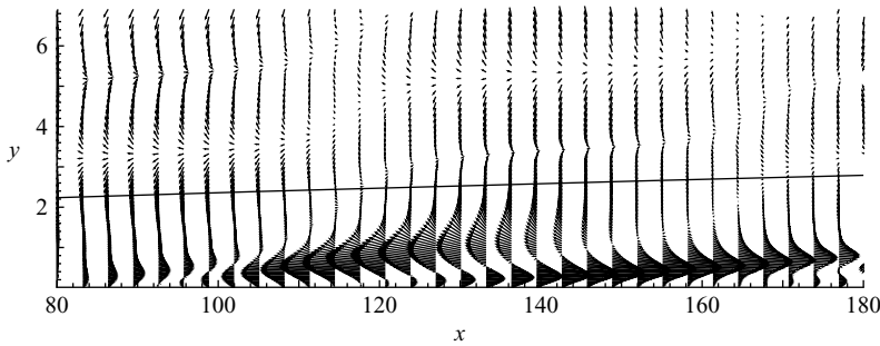
FIGURE 7. The disturbance vector of mode 2 alone; t = 3\tau .
