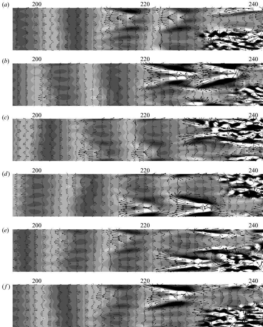
FIGURE 25. The instantaneous contour of the normal fluctuation and the vector plot of inplane components of the mode 5 case in the (x, y) -plane; y = 0.5\delta_{99} . Contours are plotted in -0.02 < v < 0.02 . Each frame is separated by \Delta t \sim 0.1\tau , where \tau is the flow-through time. The spanwise coordinate is not enlarged. The vector length is plotted as grid units magnitude = 10.
