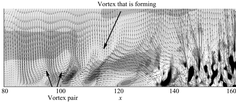
FIGURE 17. Illustration of the breakdown scenario for mode 2. An instantaneous contour of the spanwise fluctuation and with vectors of inplane components in an x - y plane.
