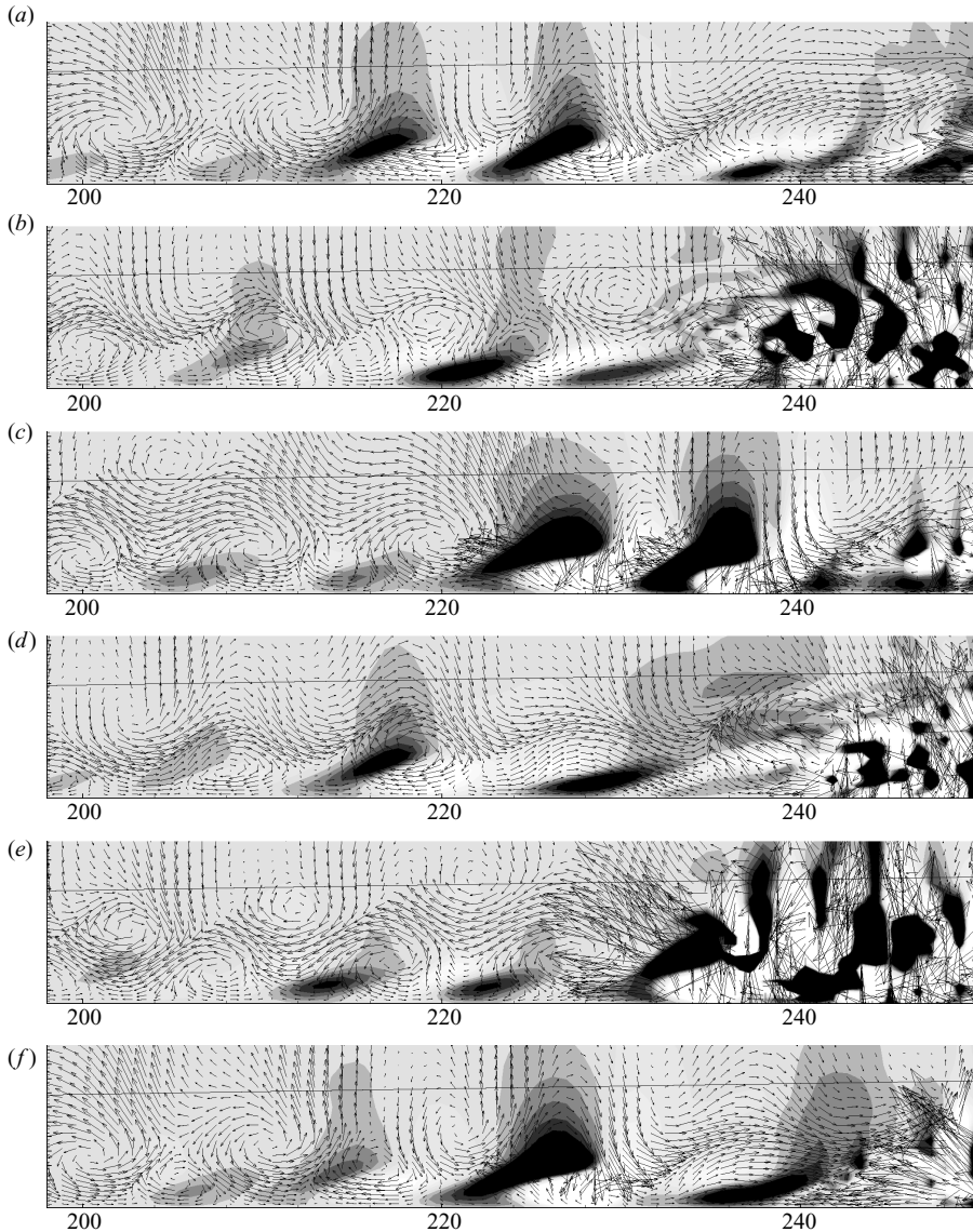
FIGURE 27. The instantaneous contour of the spanwise fluctuation and the vector plot of inplane components of the mode 5 case in the (x, y) -plane; the slice cuts through the centre of \Lambda -structures. The vector length is plotted as grid units/magnitude = 20. Snapshots are taken corresponding to figures 24 and 25.
