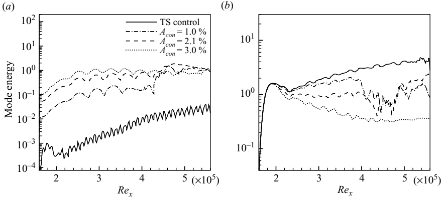
FIGURE 32. The amplitude of (a) the subharmonic and (b) first harmonic modes of the T-S perturbation.
