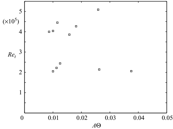
FIGURE 38. The transition Reynolds number vs. A^0_{con} \Theta .
