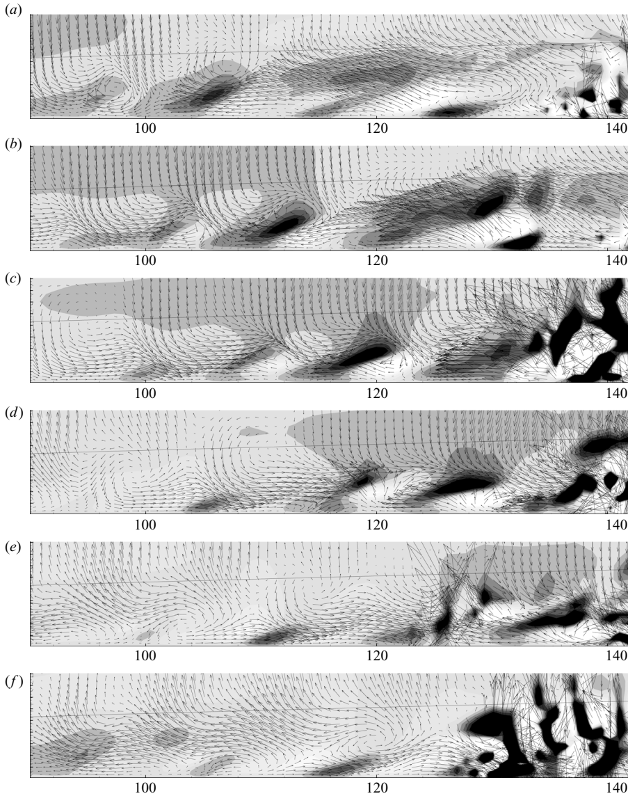
FIGURE 16. As figure 15 but the slice cuts through one leg of \Lambda -structures.
