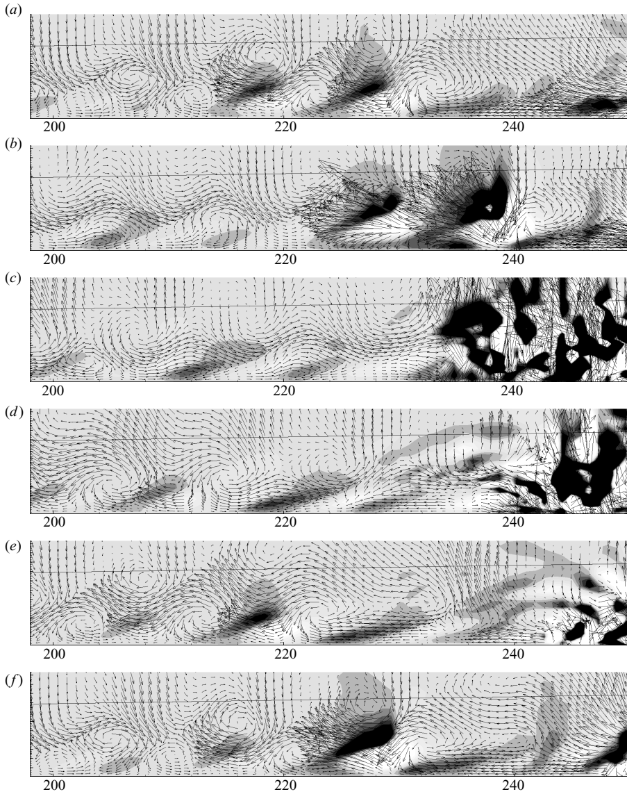
FIGURE 28. As figure 27 but the slice cuts through one leg of \Lambda -structures.
