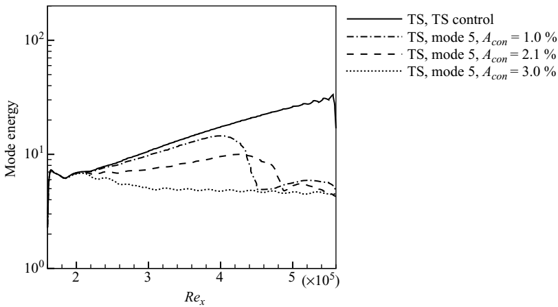
FIGURE 30. The amplitude of the fundamental T-S mode, mode 5.
