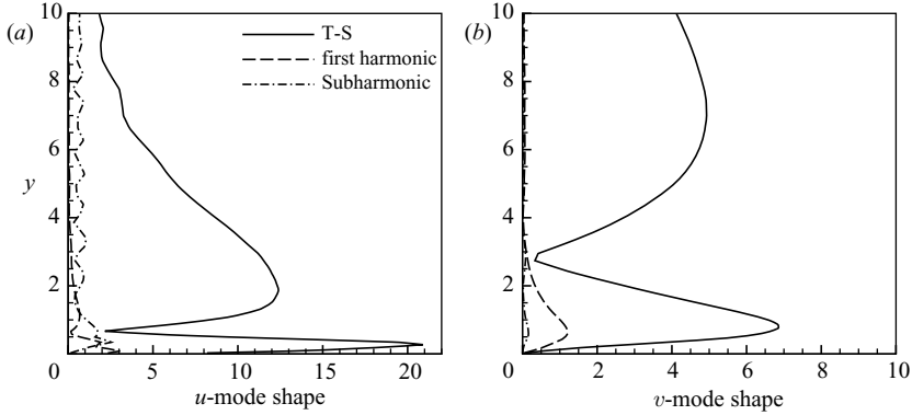
FIGURE 20. Profiles of (a) the streamwise and (b) wall-normal spectra.
