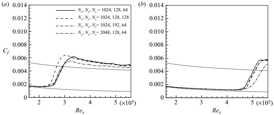
FIGURE 9. Grid resolution test: skin friction coefficient for transition due to the interaction of the T-S wave with the continuous modes (a) 2 and (b) 5.
