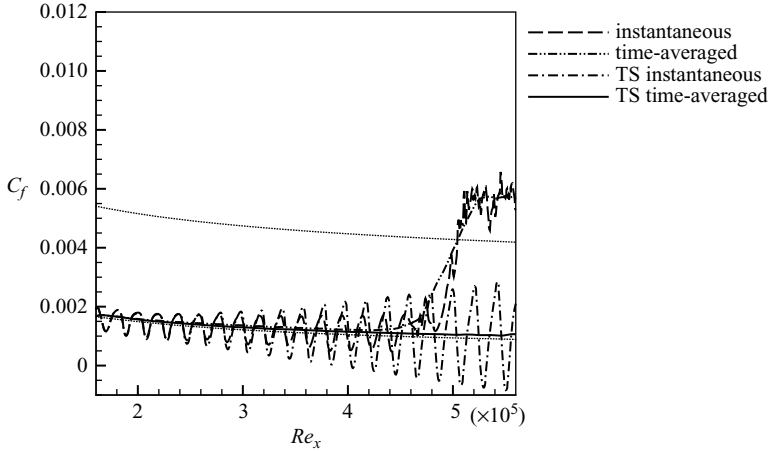
FIGURE 23. The skin friction coefficient vs. the Re_x of the mode 5 case with the T-S only case as control; t = 3\tau .
