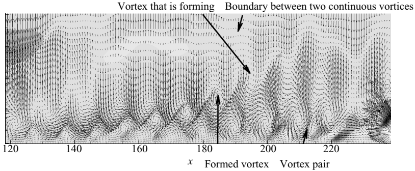
FIGURE 26. Mode 5. An instantaneous contour of the spanwise fluctuation with vectors of the inplane components in an (x, y) -plane. The vector length is plotted as grid units/magnitude = 20.
