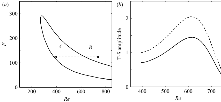
FIGURE 3. (a) The neutral curve for a zero-pressure gradient boundary layer (Bertolotti, Herbert & Spalart 1992). A and B mark the inlet and exit conditions for the T-S wave. (b) The downstream evolution of the u -perturbation. —, \max(u_{rms}(y)) ; - - -, \max(u(y, t)) = \sqrt{2}\max(u_{rms}) .
