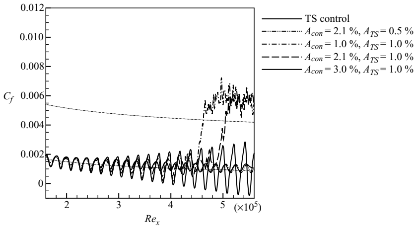
FIGURE 29. The skin friction of mode 5; effects of disturbance energy.
